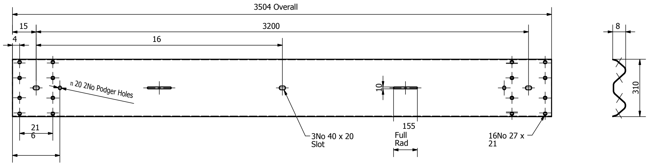
C01 Beam
